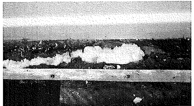
Photo 9: other cracks remain as at the first inspection
