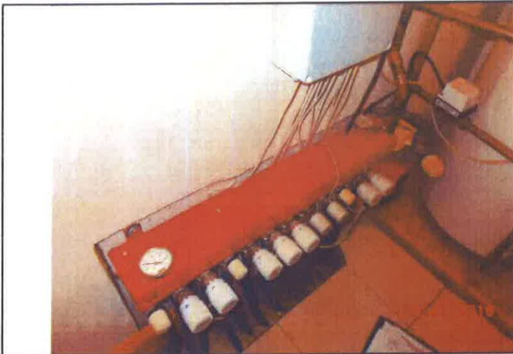
1. General view of heating system manifold (new valves are 8th and 9th from left)
