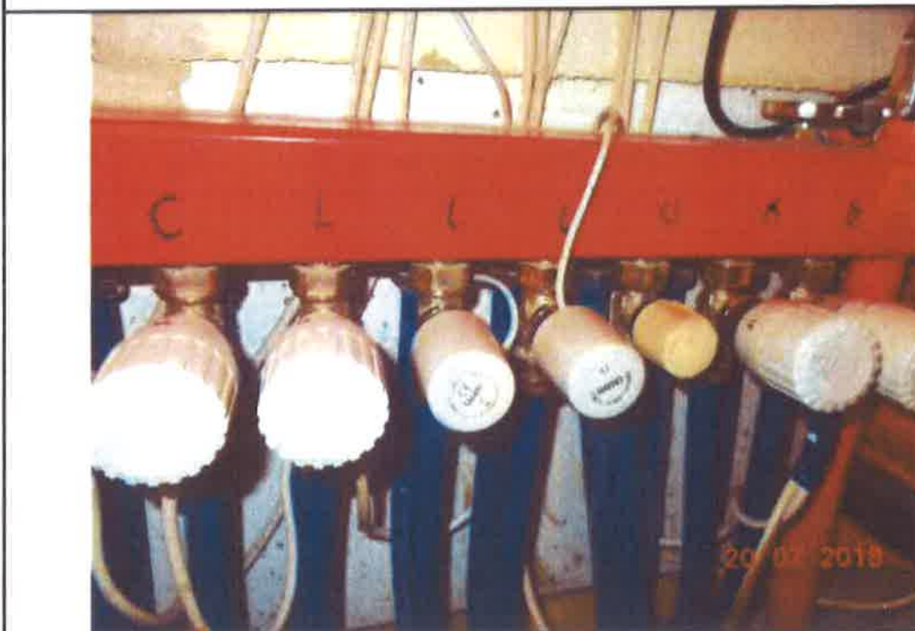
2. Close up of new valves on heating manifold (3rd and 4th from left)
